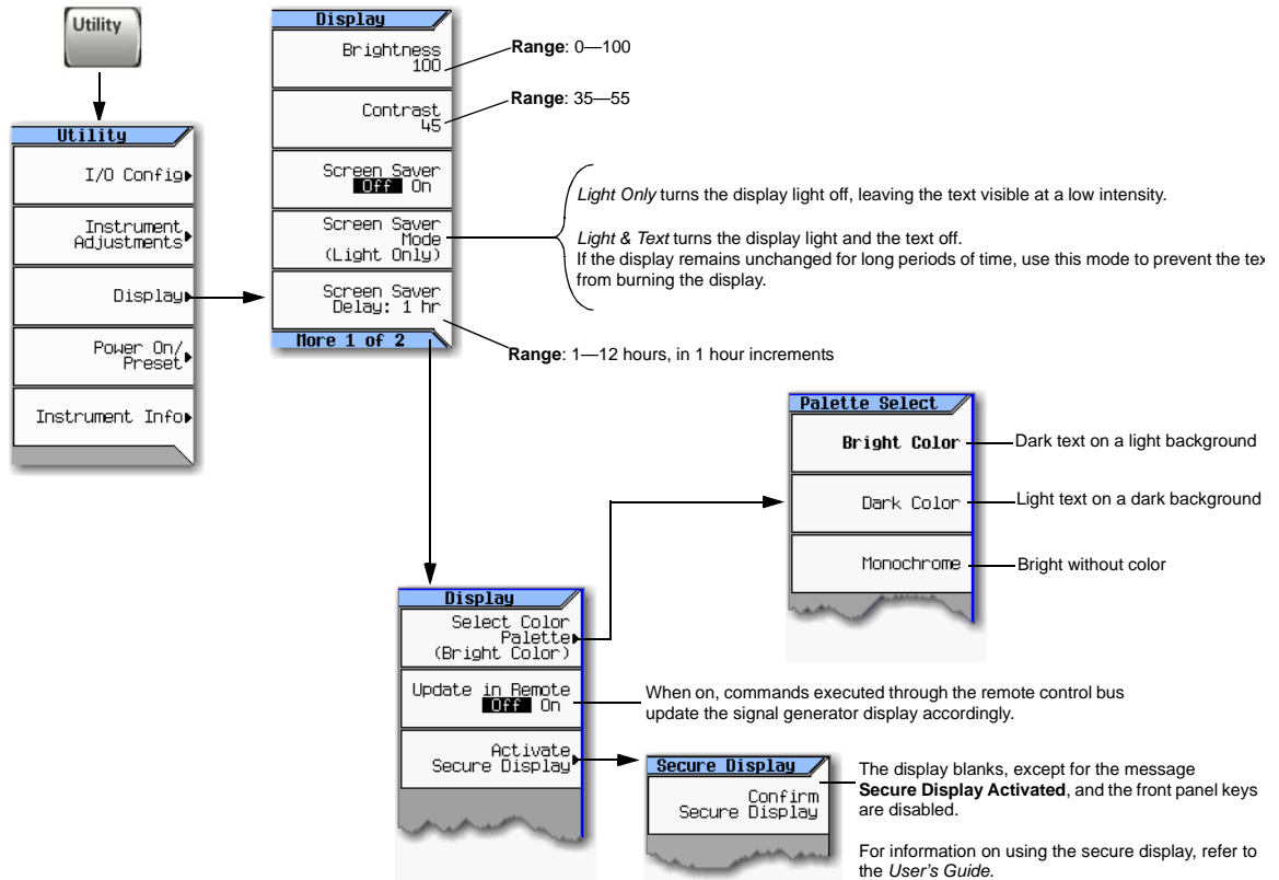
Figure 2-1 Display Softkeys
